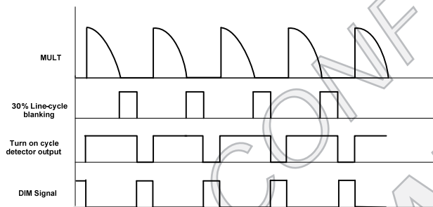
Figure 17: Dim Signal Logic
