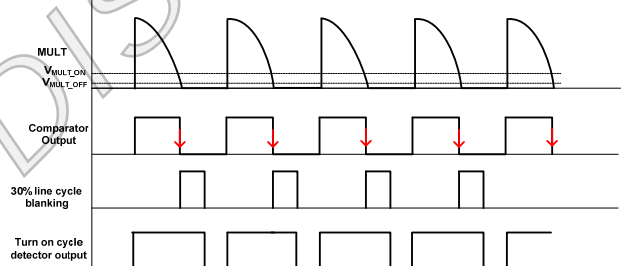
Figure 12: Dimming Turn-On Cycle Detector
