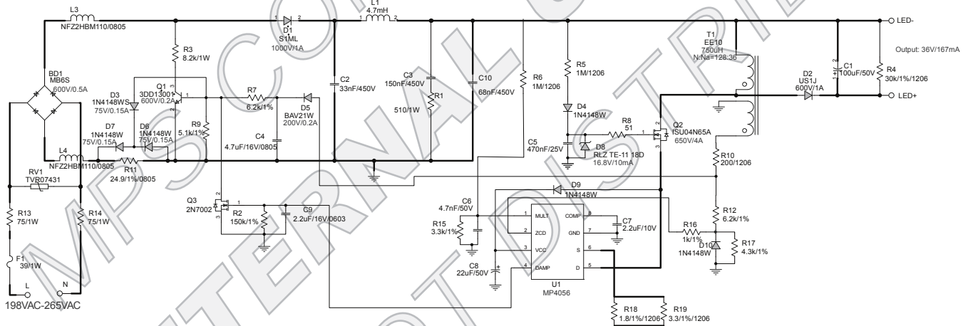
Figure 21: GU10 Bulb Driver, 230VAC/50Hz Input, V_O = 36V , I_O = 167mA , Buck-Boost Converter, High Performance, EVB Model: EV4056-S-00B
