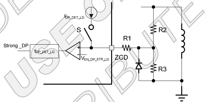
Figure 15: Weak/Strong Dimming Pull Down Current Source Selection
