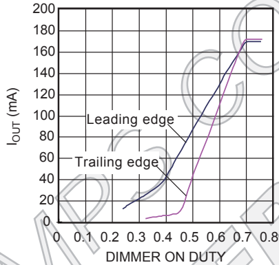
Dimming Curve
