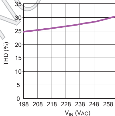
THD vs. V IN
