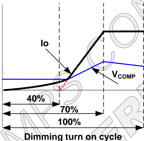
Figure 14: Trailing Edge Dimming Curve
