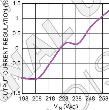
Line Regulator
